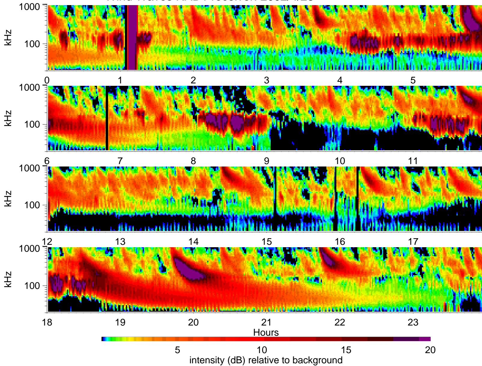
Wind Waves RAD1 receiver: 2002/4/28
