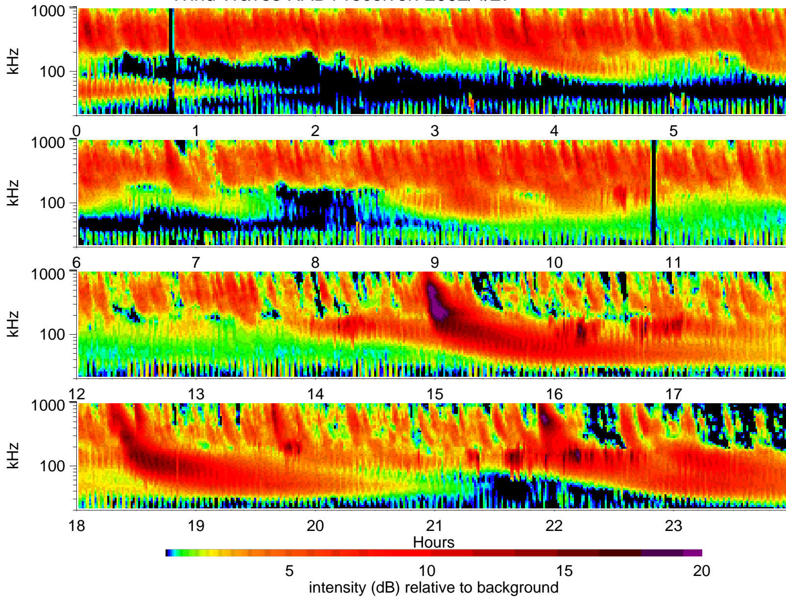
Wind Waves RAD1 receiver: 2002/4/27
