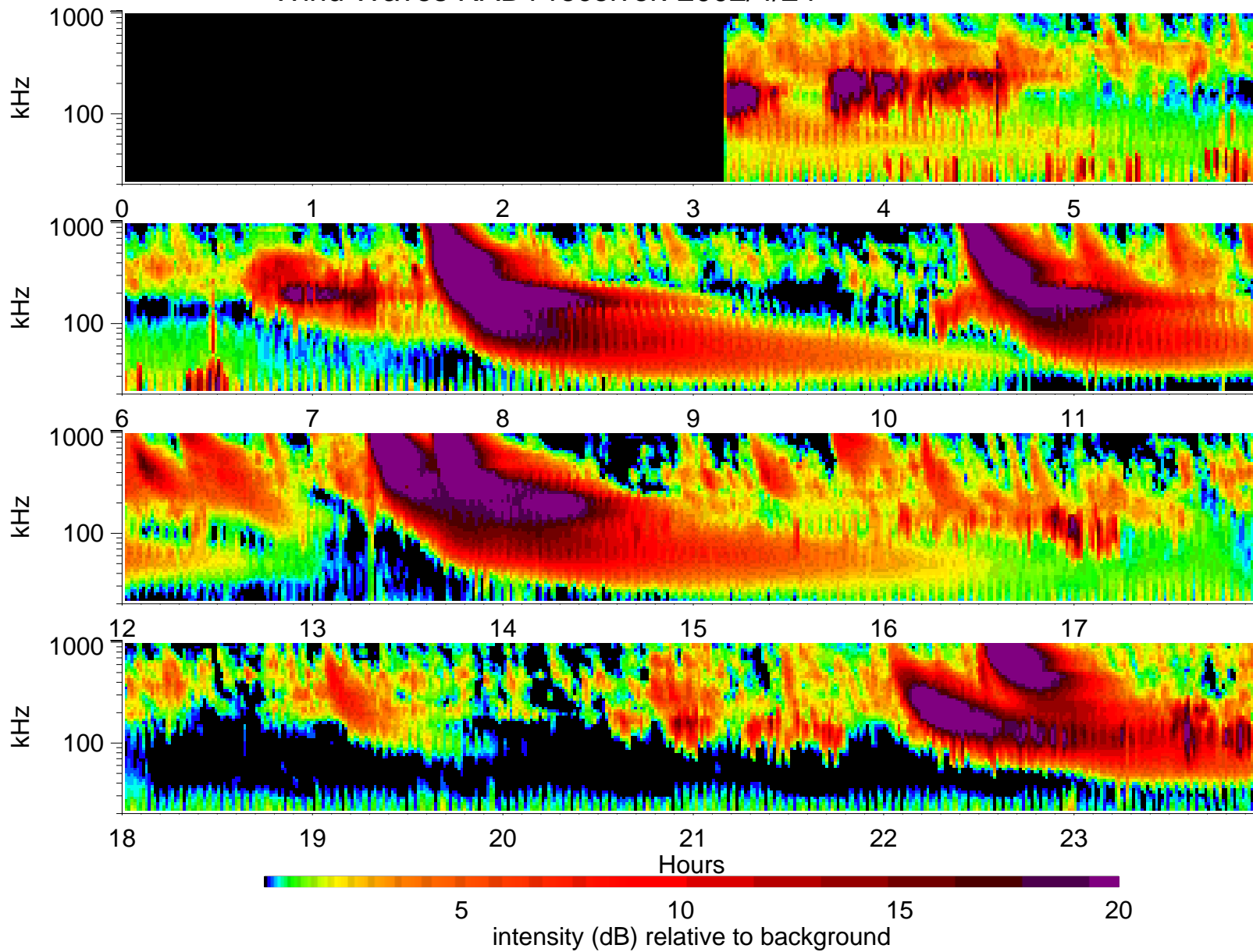
Wind Waves RAD1 receiver: 2002/4/24
