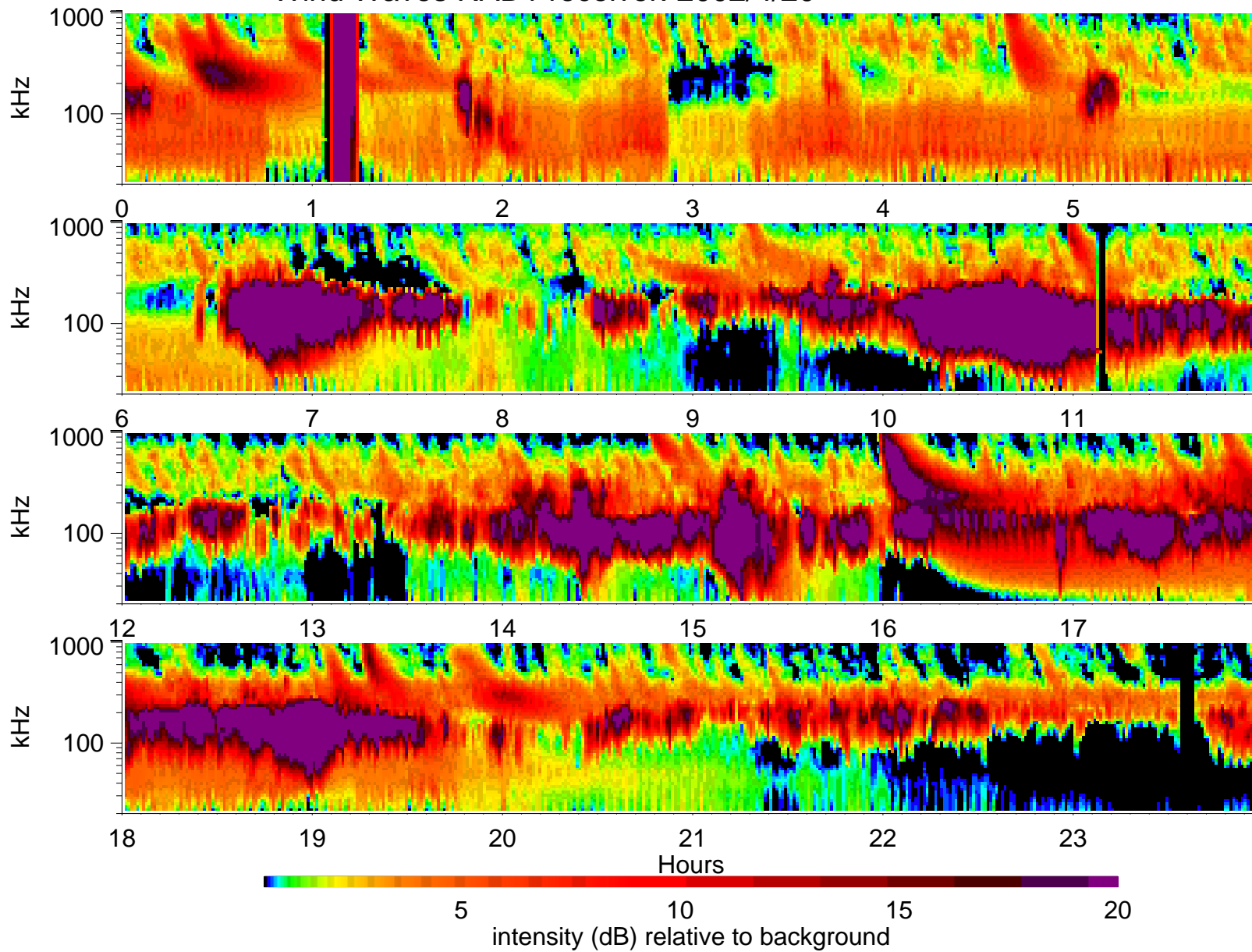
Wind Waves RAD1 receiver: 2002/4/20
