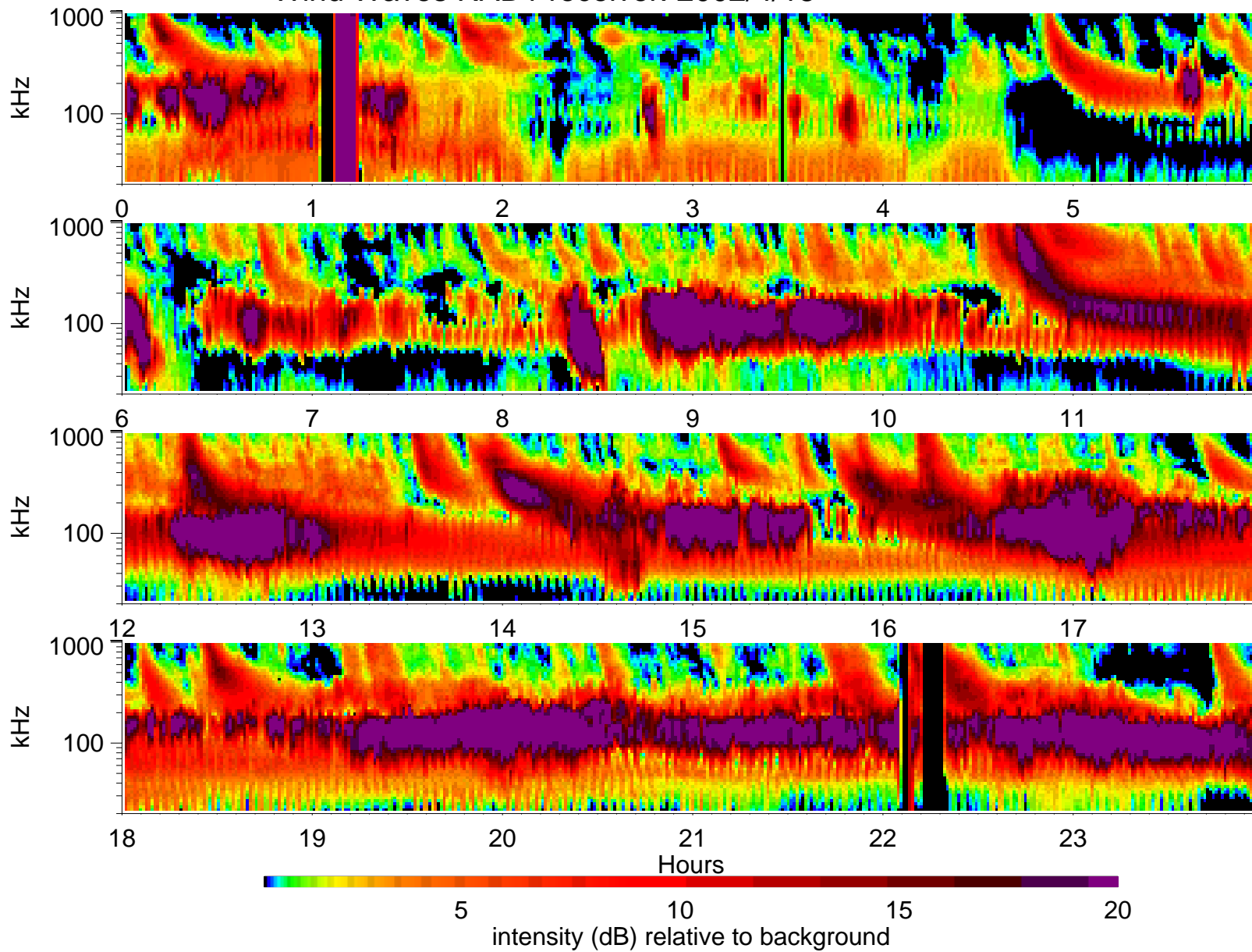
Wind Waves RAD1 receiver: 2002/4/18
