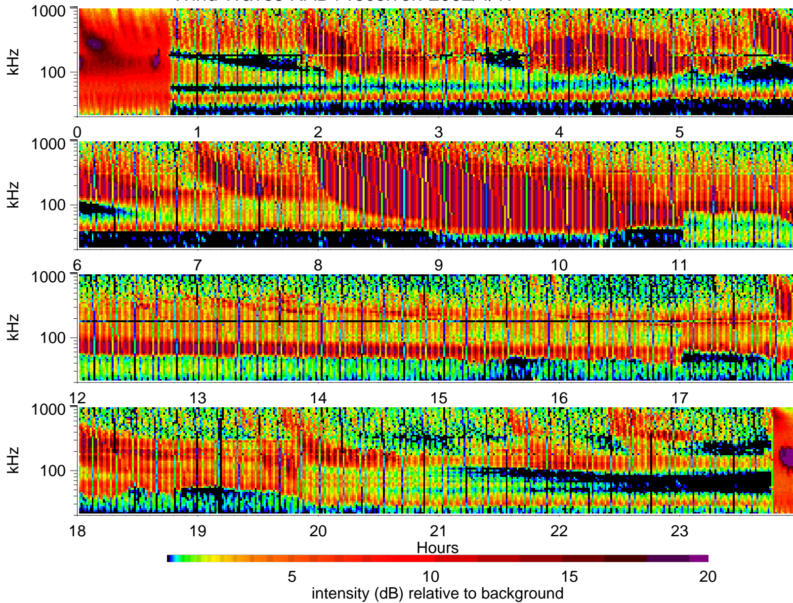
Wind Waves RAD1 receiver: 2002/4/17
