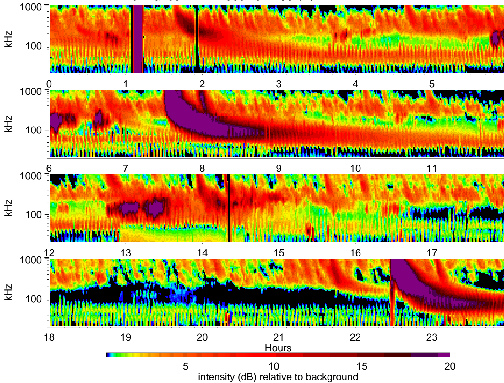
Wind Waves RAD1 receiver: 2002/4/14
