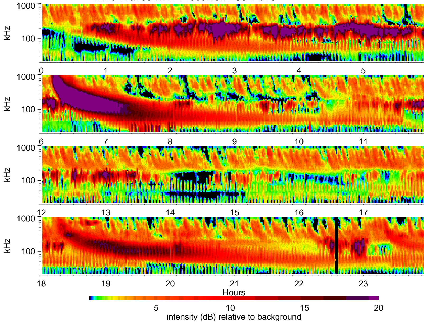
Wind Waves RAD1 receiver: 2002/4/13
