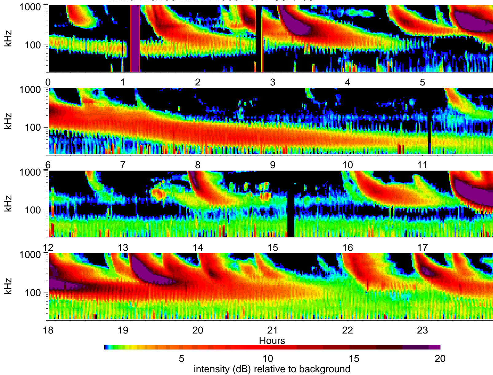
Wind Waves RAD1 receiver: 2002/4/8
