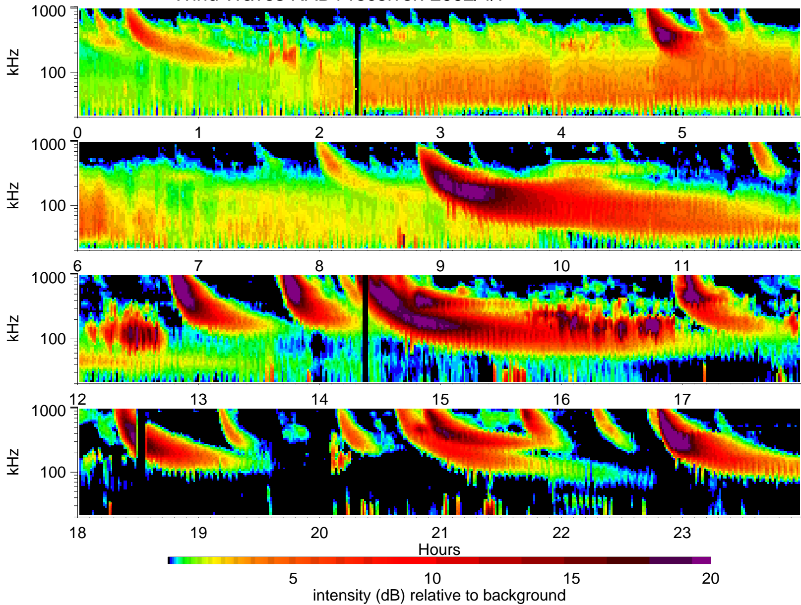
Wind Waves RAD1 receiver: 2002/4/7
