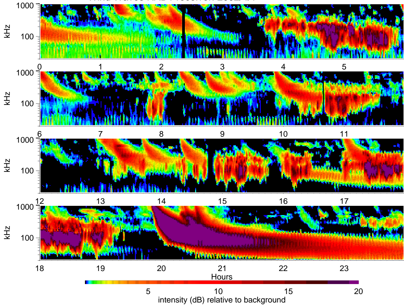
Wind Waves RAD1 receiver: 2002/4/1
