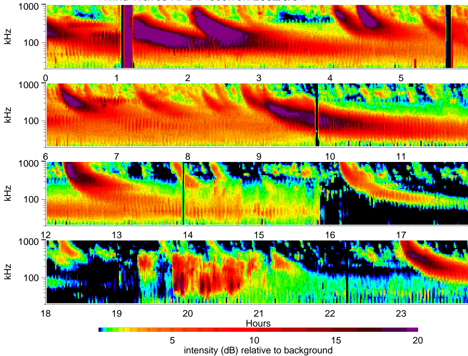
Wind Waves RAD1 receiver: 2002/3/31
