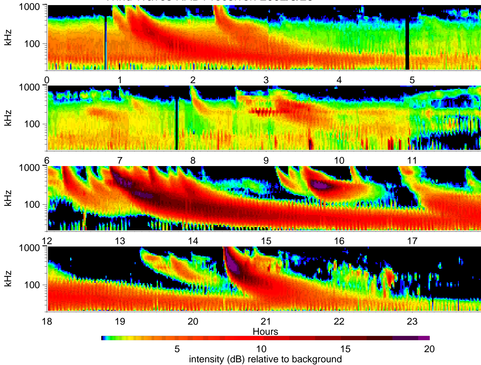
Wind Waves RAD1 receiver: 2002/3/26
