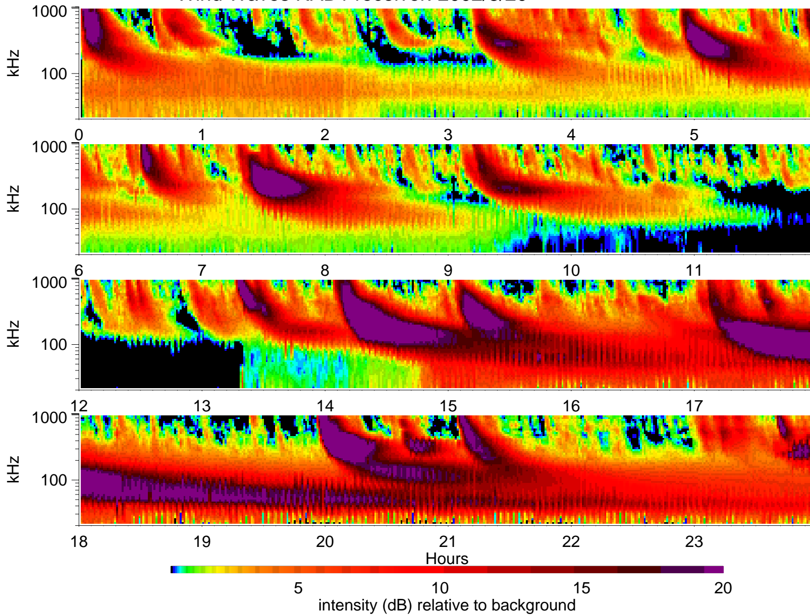
Wind Waves RAD1 receiver: 2002/3/20
