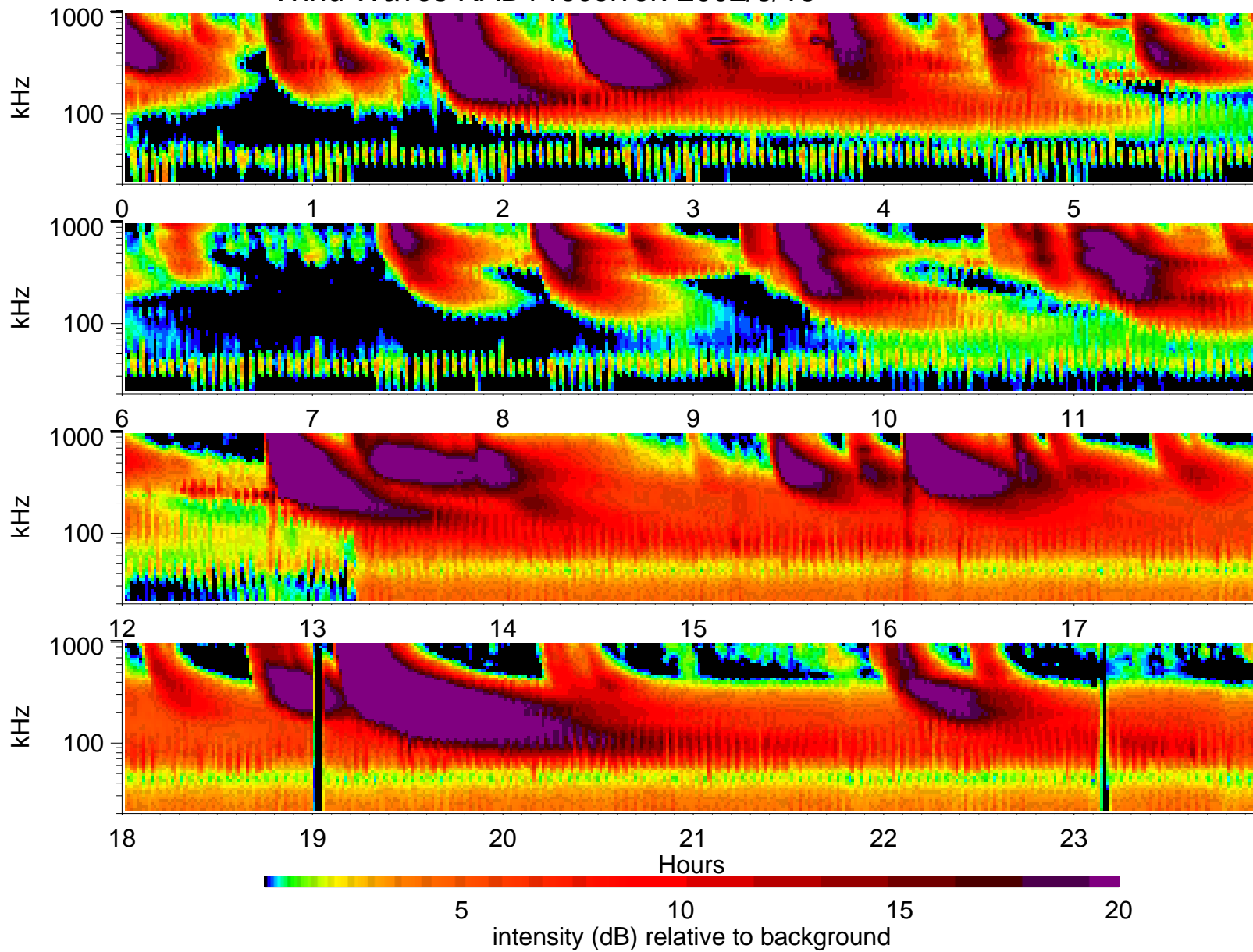
Wind Waves RAD1 receiver: 2002/3/18
