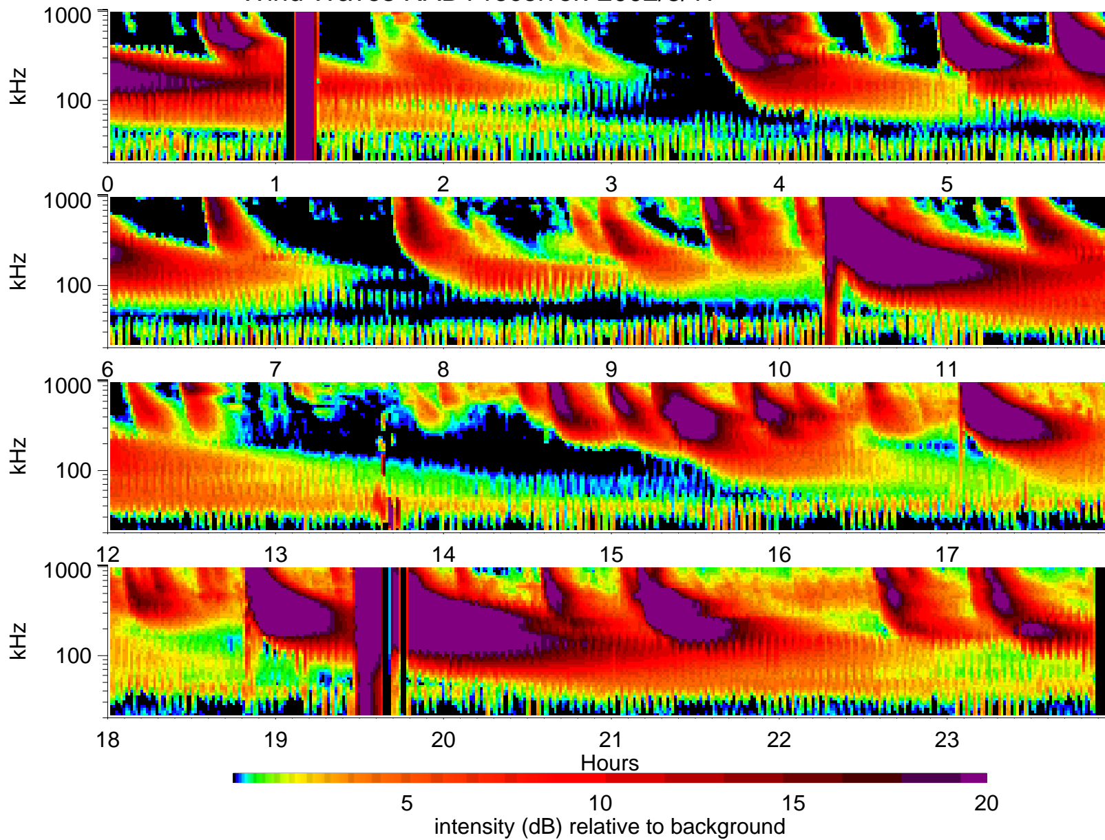
Wind Waves RAD1 receiver: 2002/3/17
