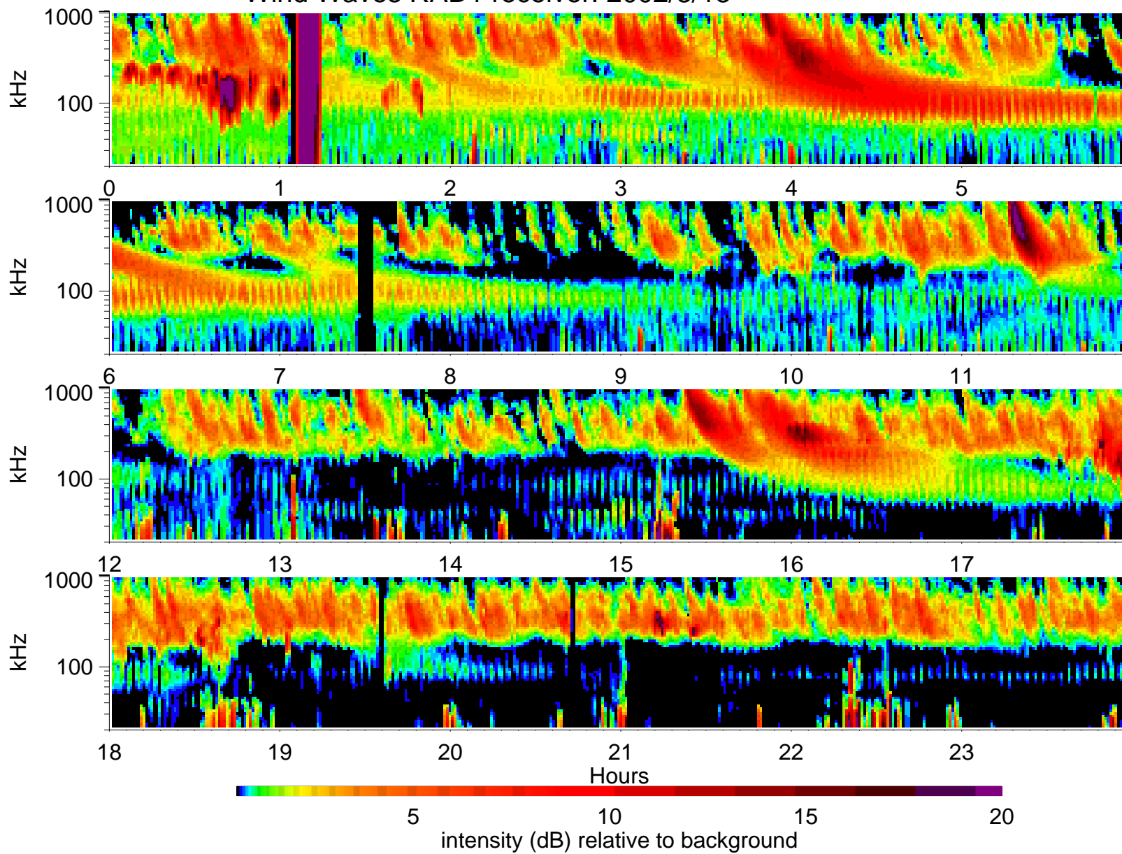
Wind Waves RAD1 receiver: 2002/3/13
