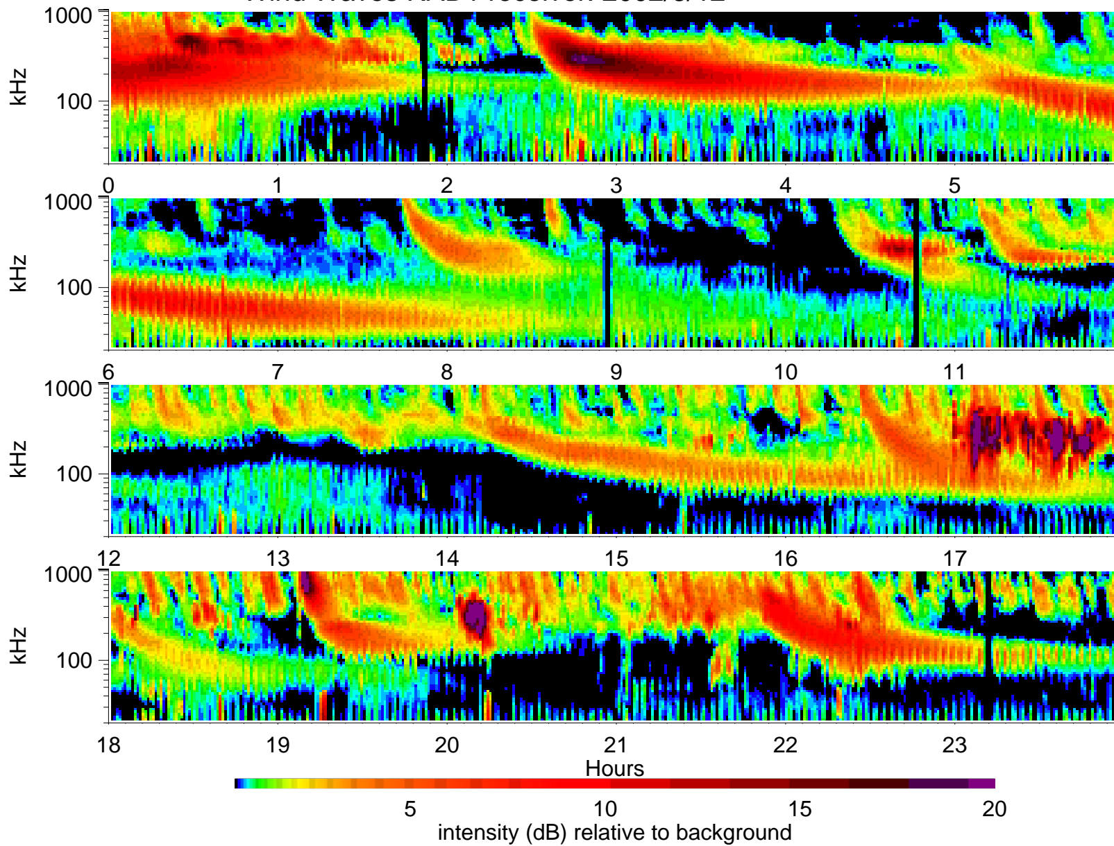
Wind Waves RAD1 receiver: 2002/3/12
