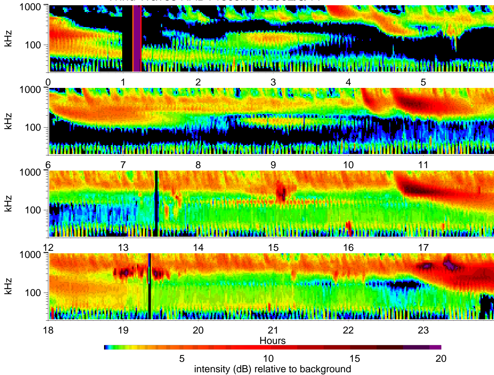
Wind Waves RAD1 receiver: 2002/3/11
