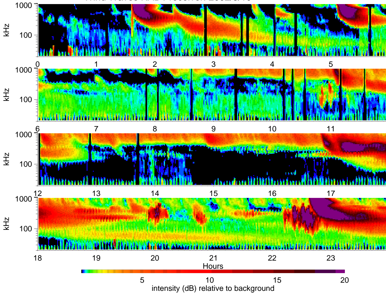
Wind Waves RAD1 receiver: 2002/3/10
