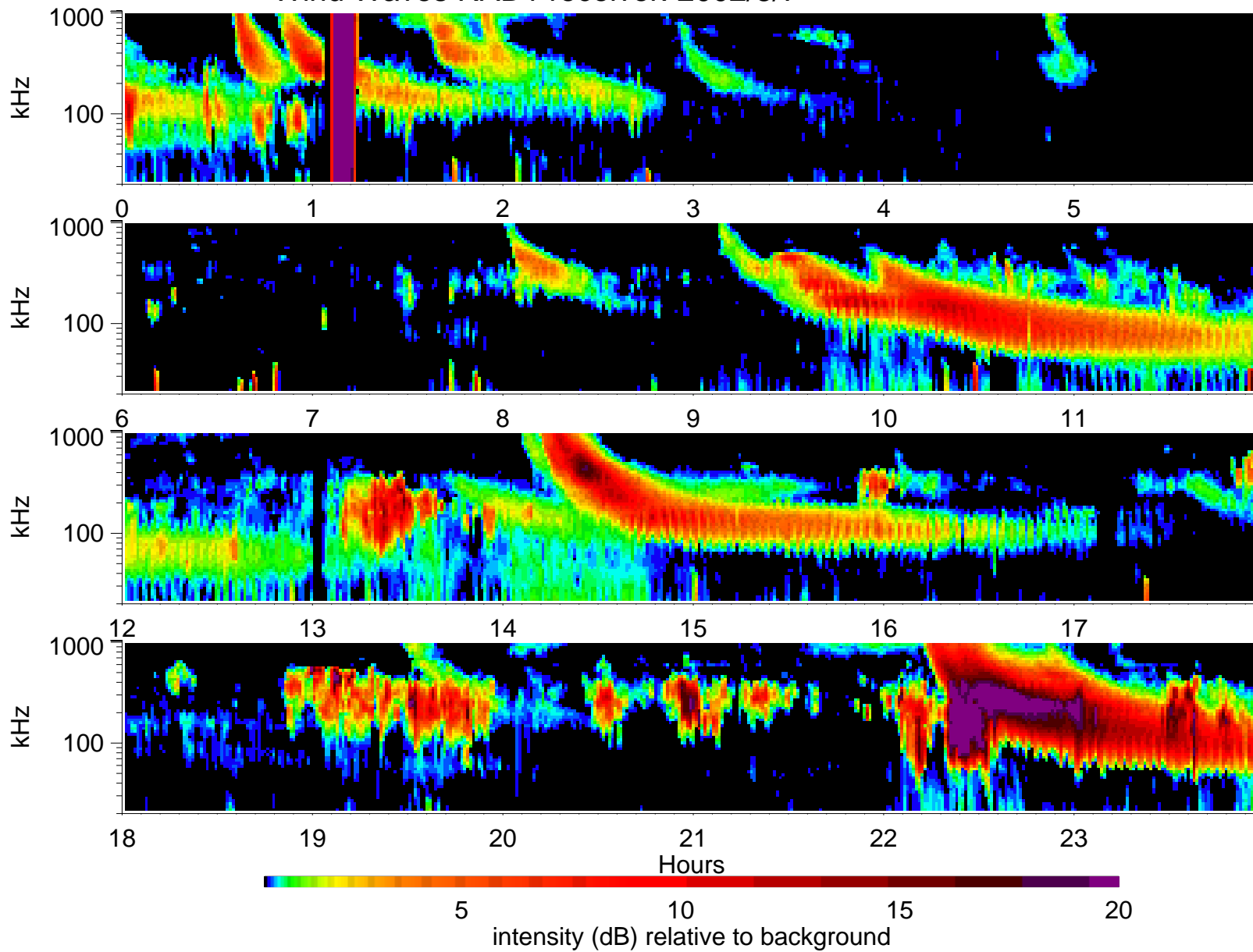
Wind Waves RAD1 receiver: 2002/3/7
