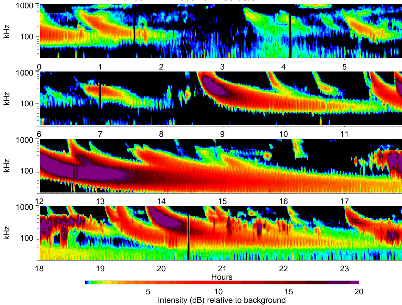
Wind Waves RAD1 receiver: 2002/3/6
