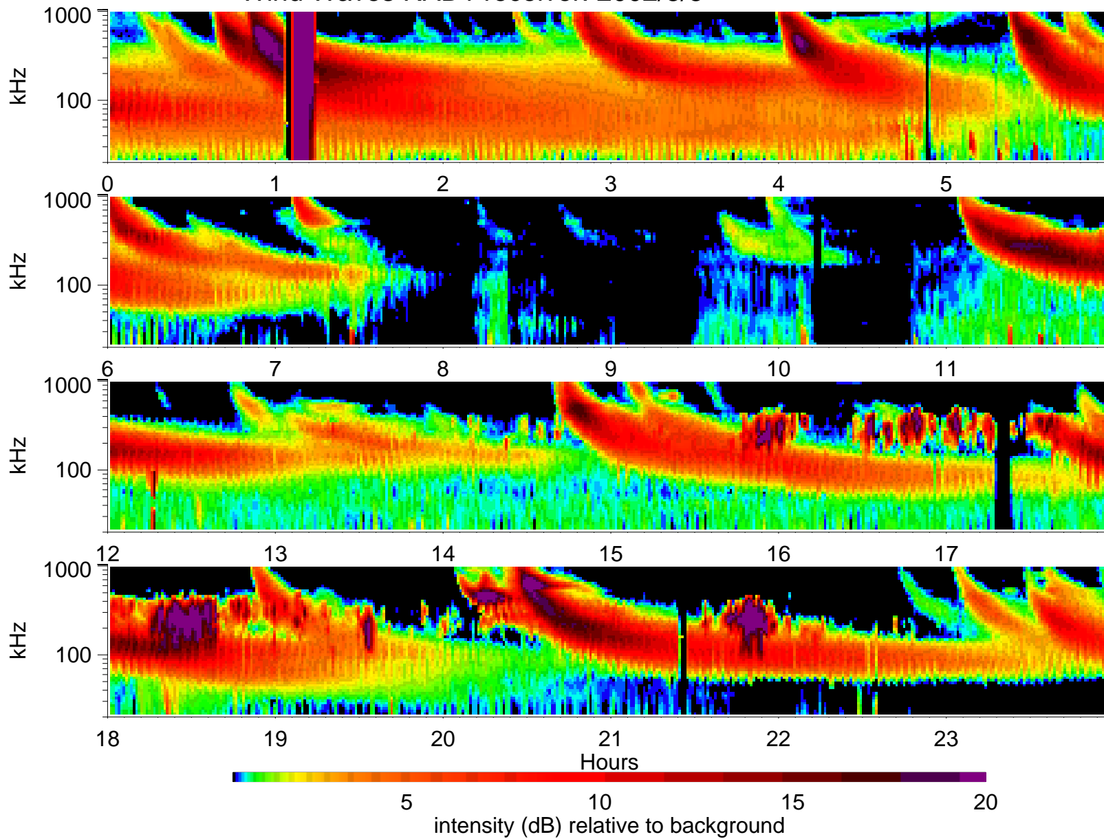
Wind Waves RAD1 receiver: 2002/3/5
