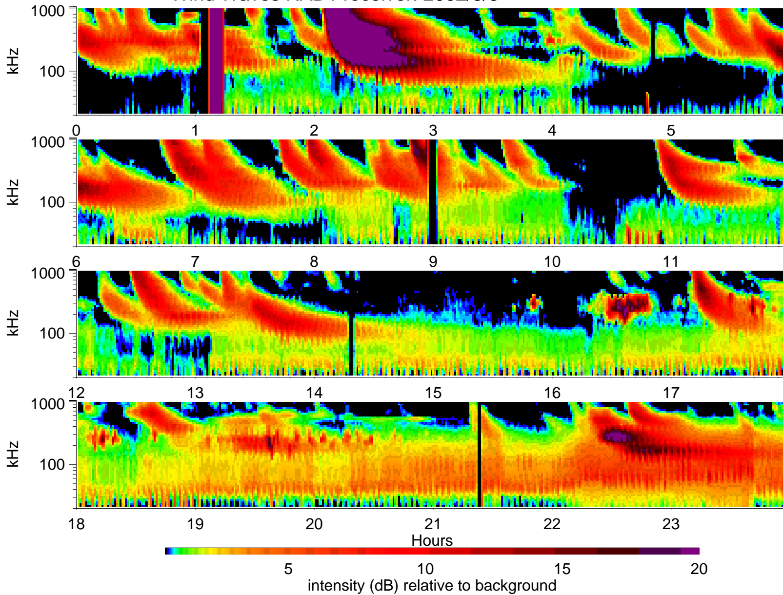
Wind Waves RAD1 receiver: 2002/3/3
