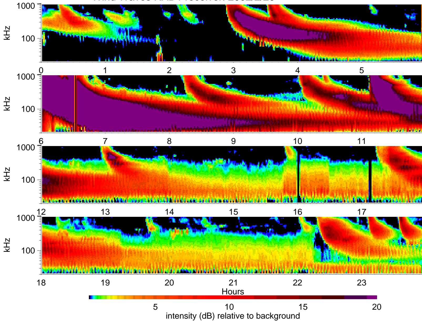
Wind Waves RAD1 receiver: 2002/2/20
