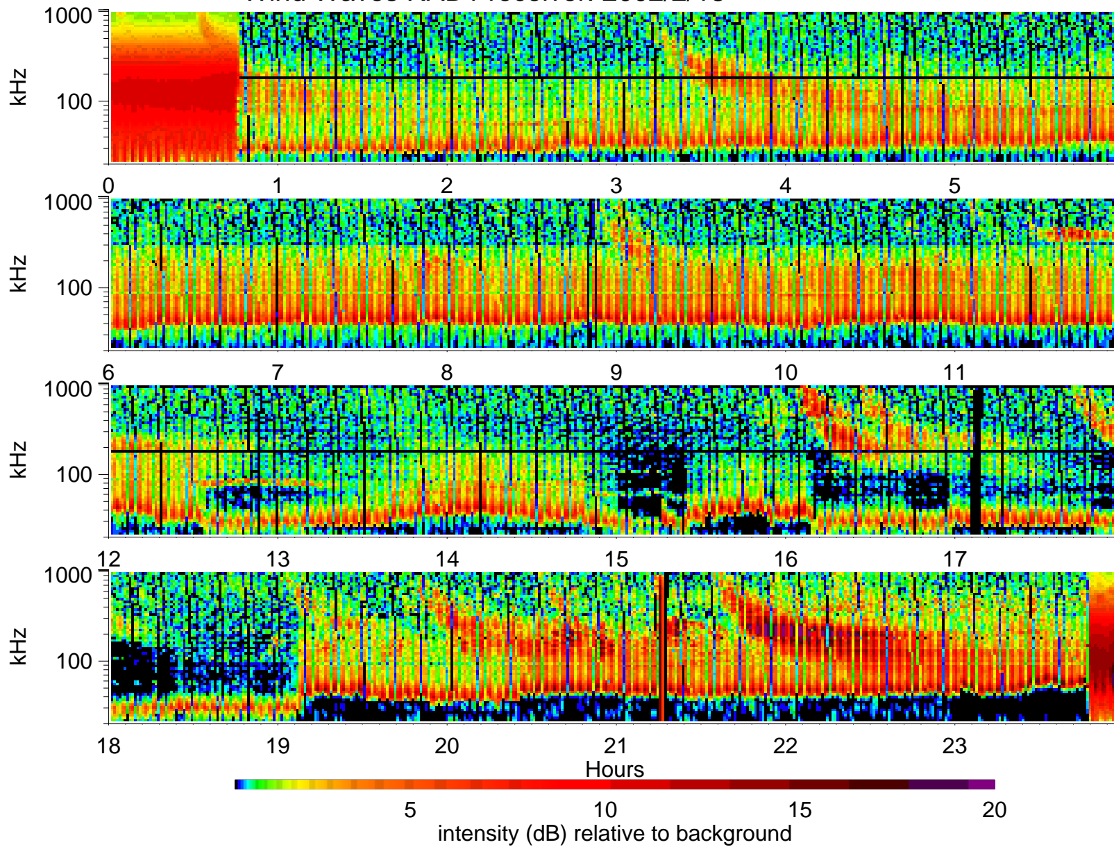
Wind Waves RAD1 receiver: 2002/2/18
