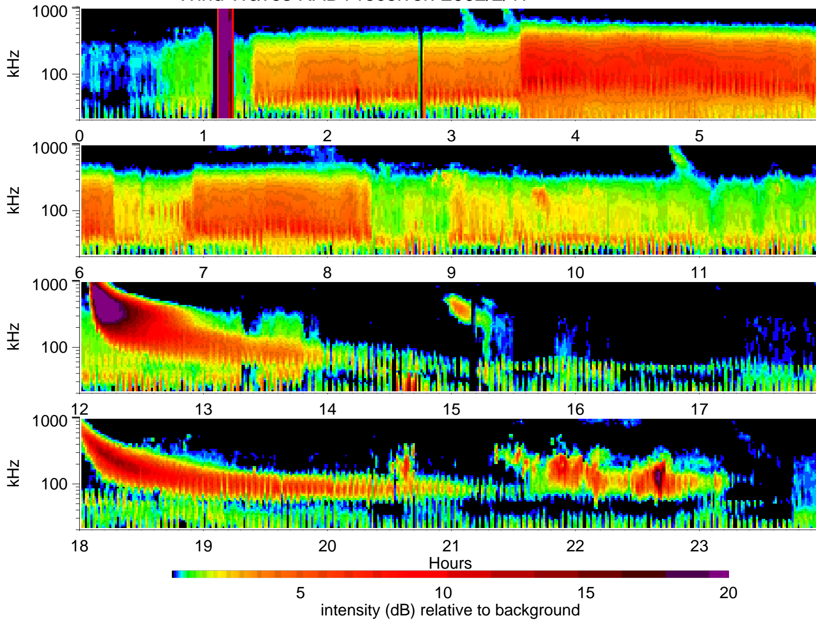
Wind Waves RAD1 receiver: 2002/2/17
