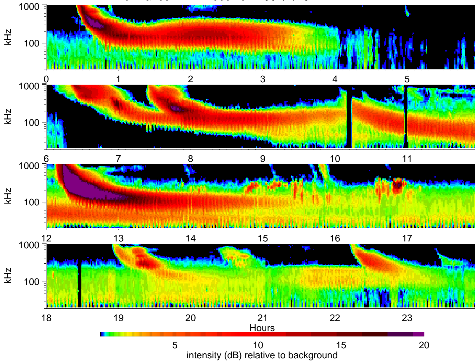
Wind Waves RAD1 receiver: 2002/2/16
