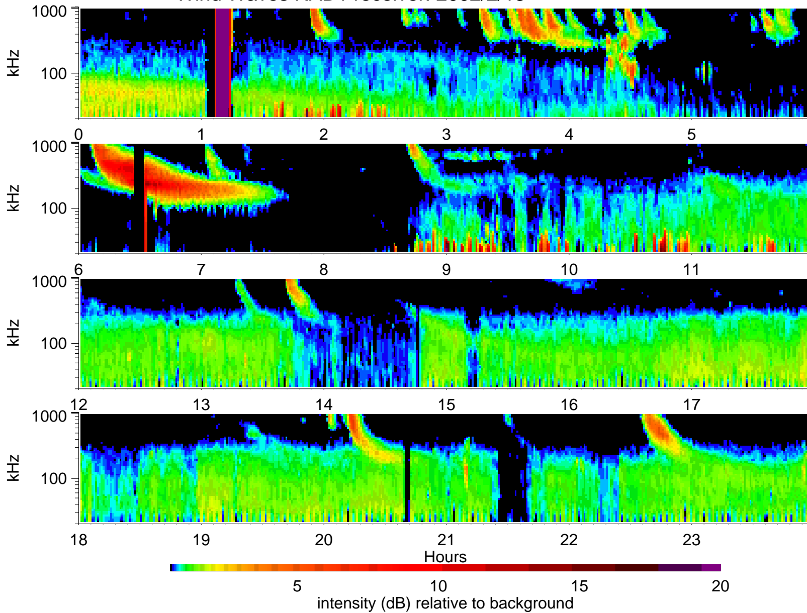
Wind Waves RAD1 receiver: 2002/2/15
