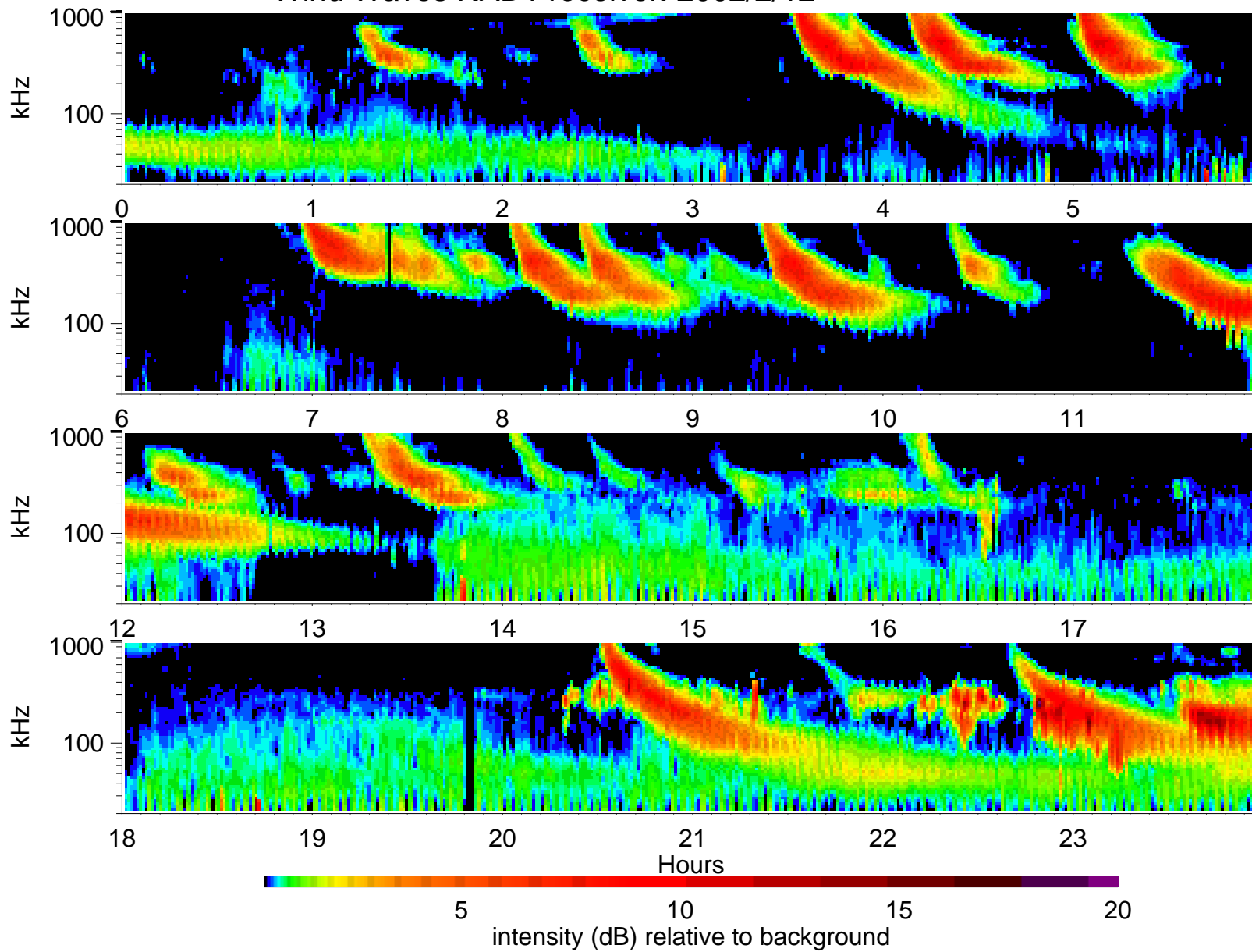
Wind Waves RAD1 receiver: 2002/2/12
