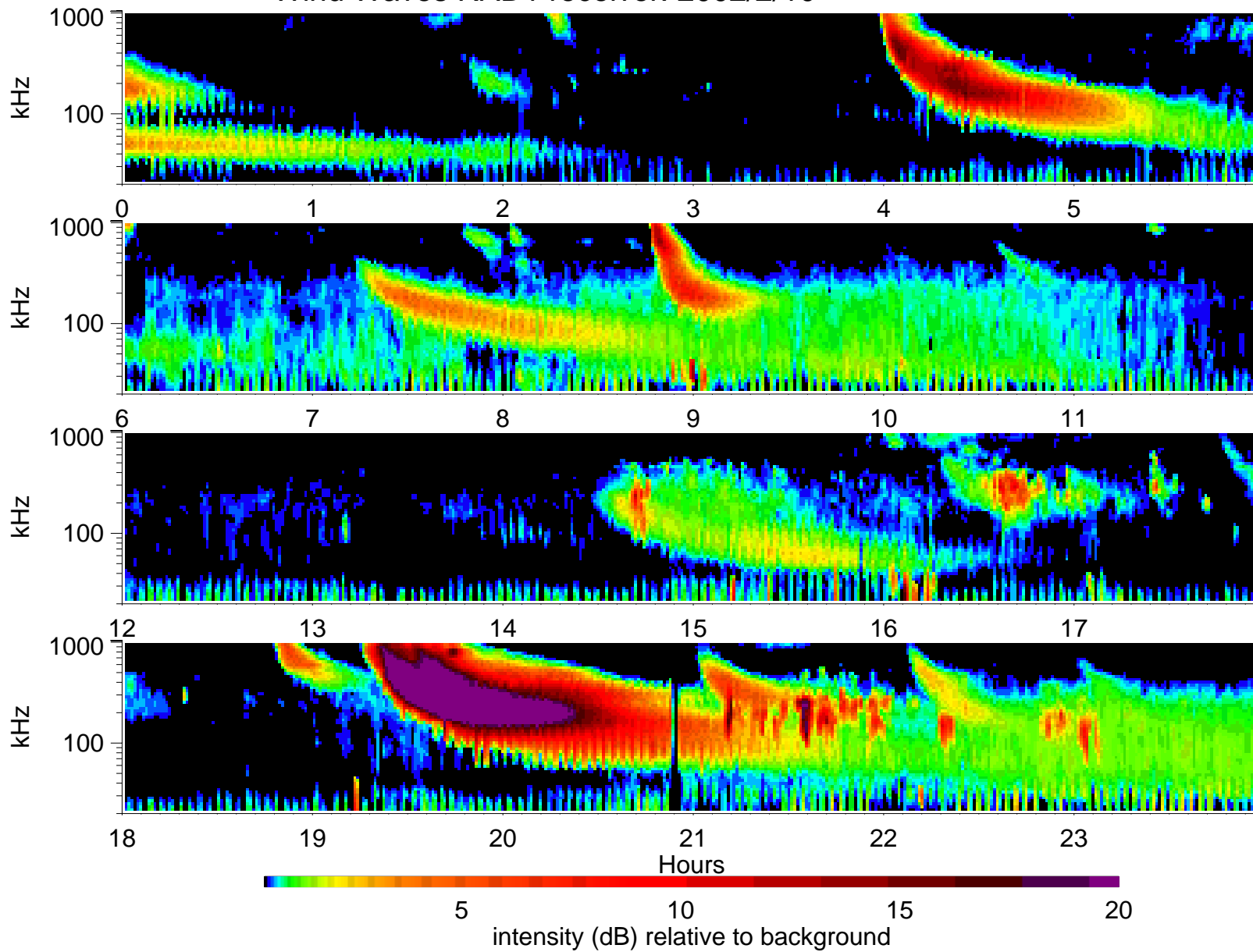
Wind Waves RAD1 receiver: 2002/2/10
