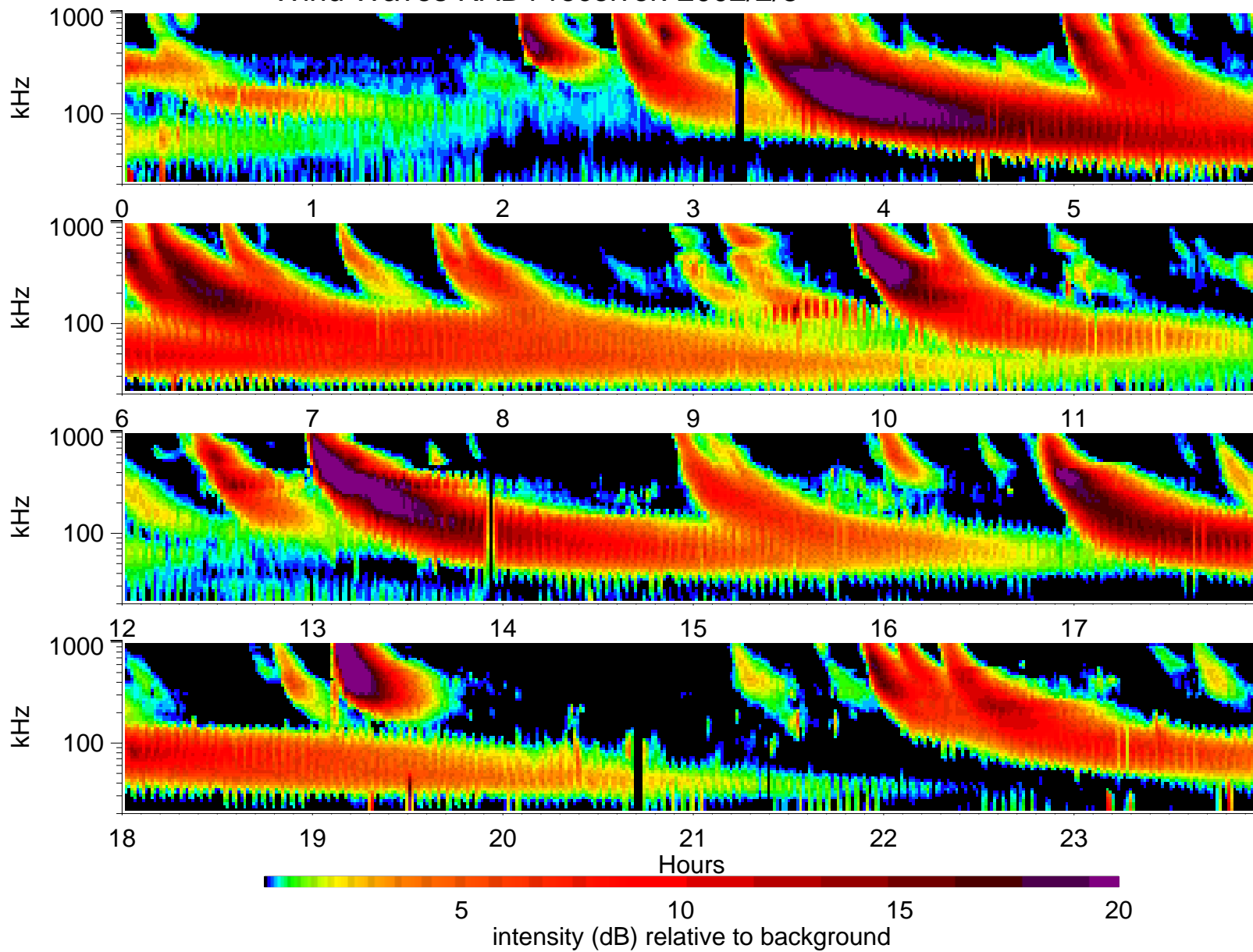
Wind Waves RAD1 receiver: 2002/2/8
