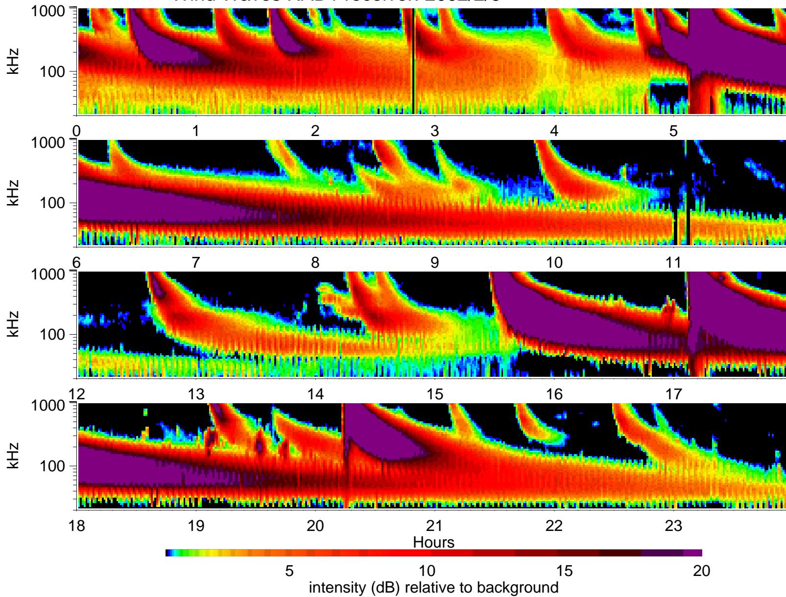
Wind Waves RAD1 receiver: 2002/2/6
