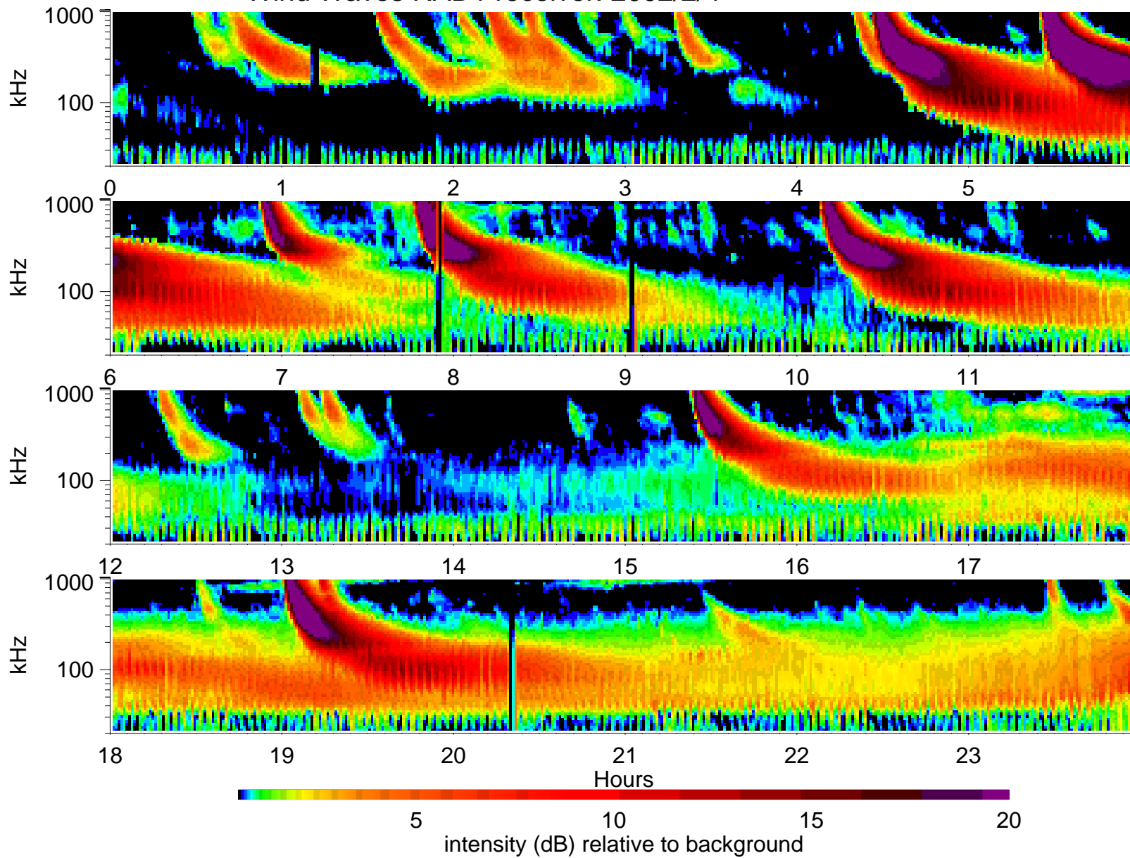
Wind Waves RAD1 receiver: 2002/2/4
