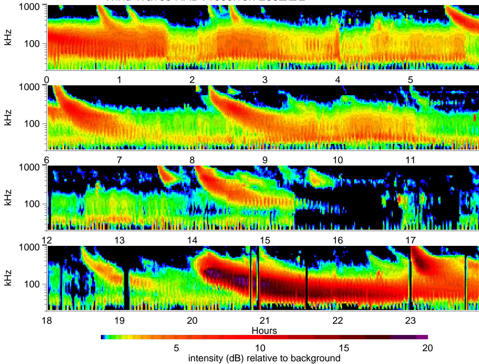
Wind Waves RAD1 receiver: 2002/2/2
