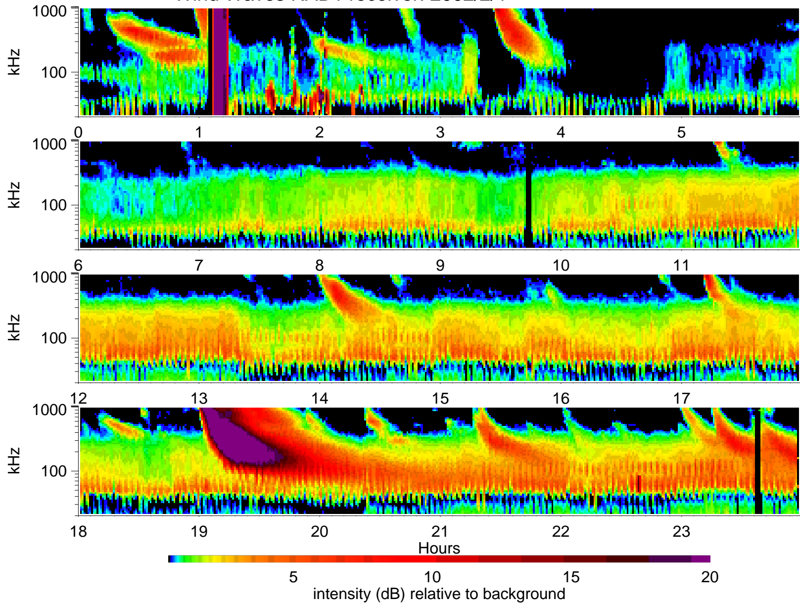
Wind Waves RAD1 receiver: 2002/2/1
