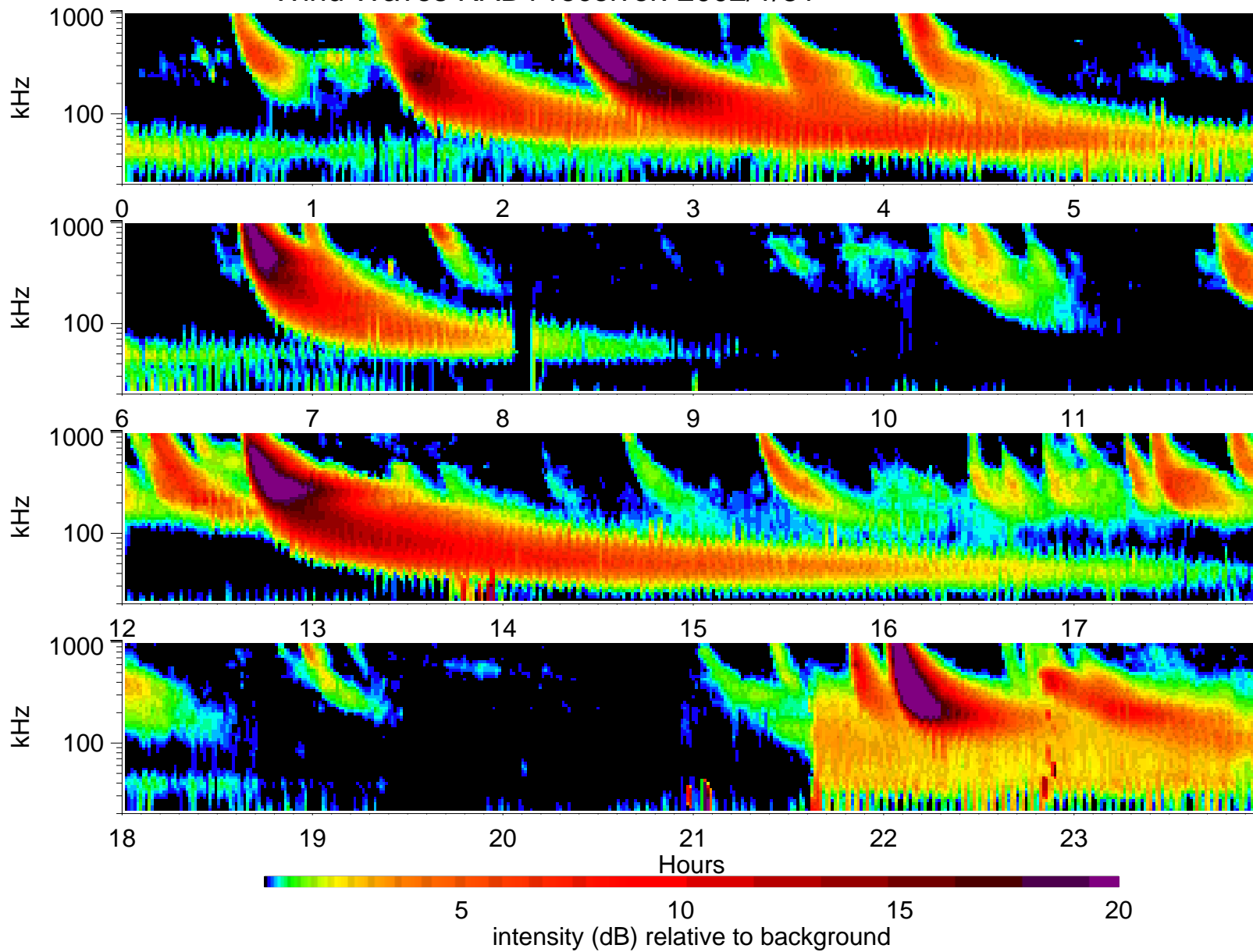
Wind Waves RAD1 receiver: 2002/1/31
