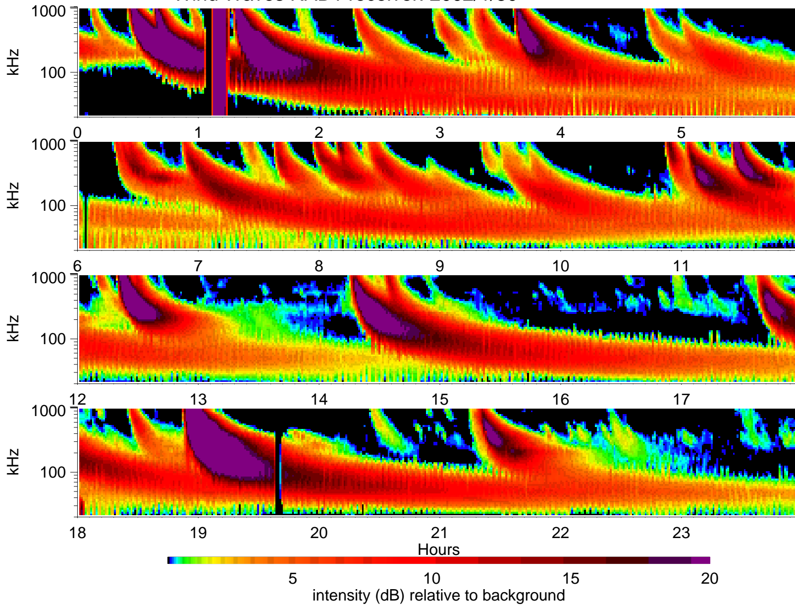
Wind Waves RAD1 receiver: 2002/1/30
