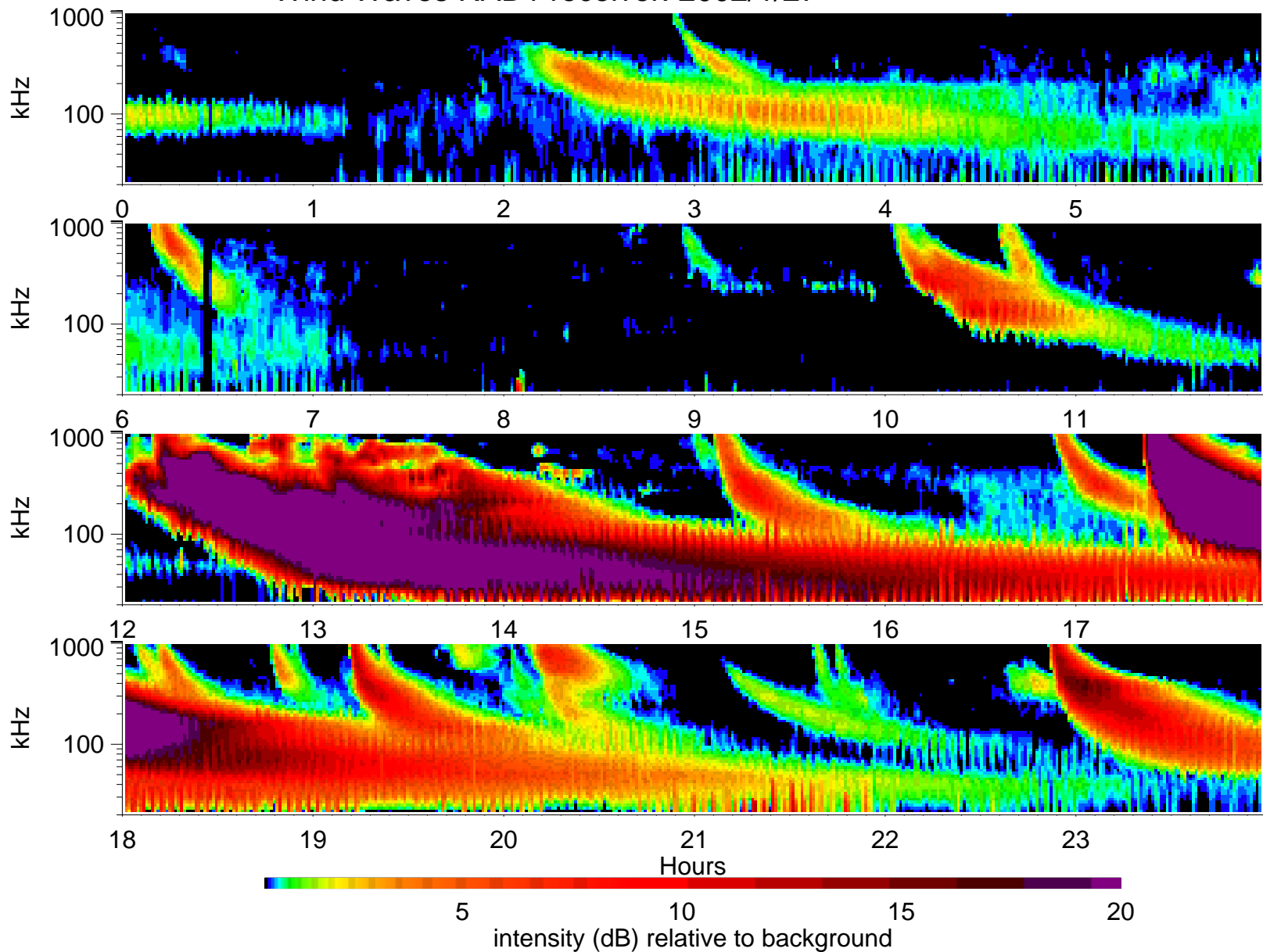
Wind Waves RAD1 receiver: 2002/1/27
