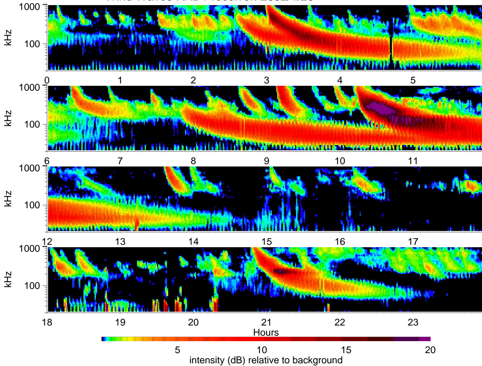
Wind Waves RAD1 receiver: 2002/1/23
