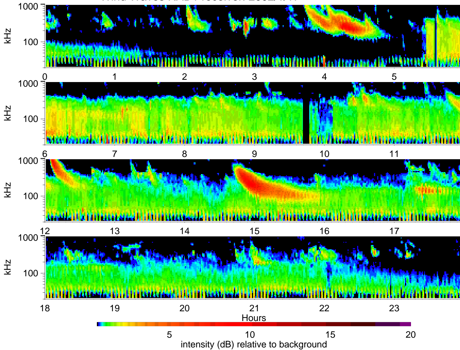
Wind Waves RAD1 receiver: 2002/1/17
