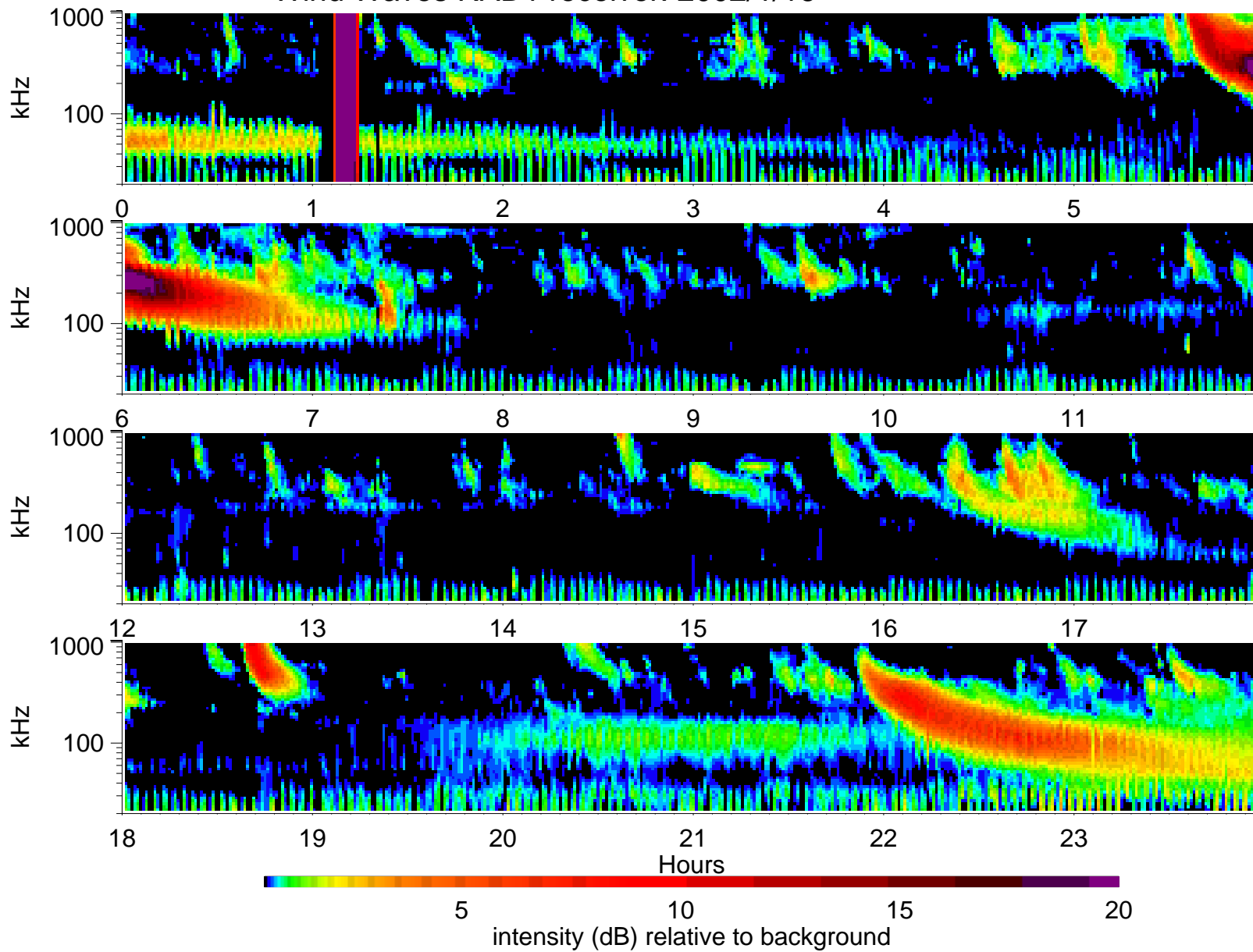
Wind Waves RAD1 receiver: 2002/1/16
