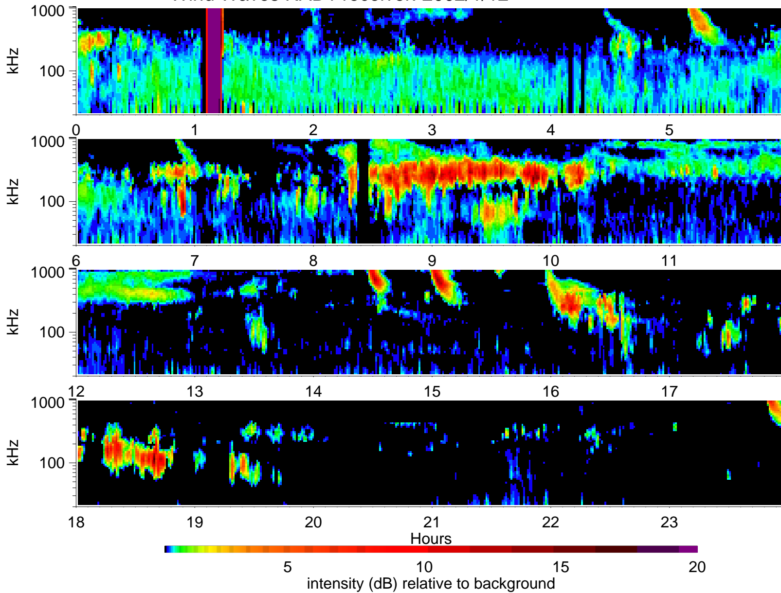
Wind Waves RAD1 receiver: 2002/1/12
