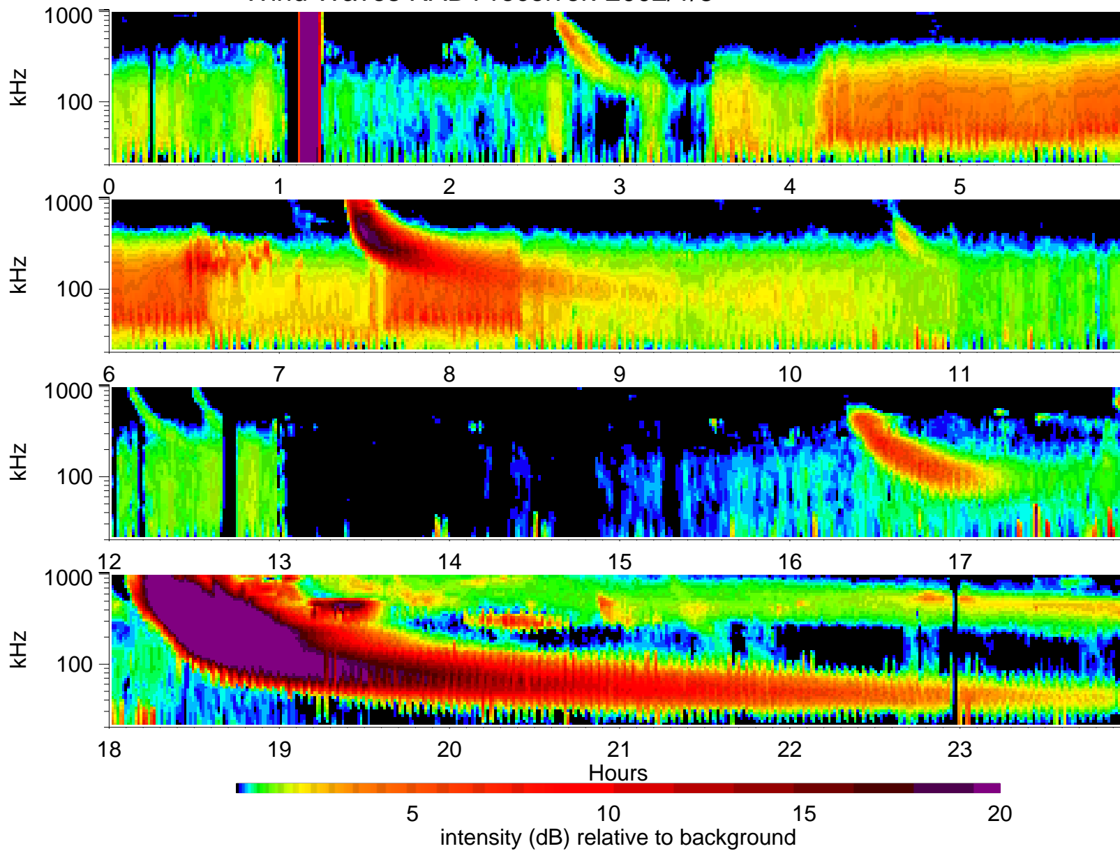
Wind Waves RAD1 receiver: 2002/1/8
