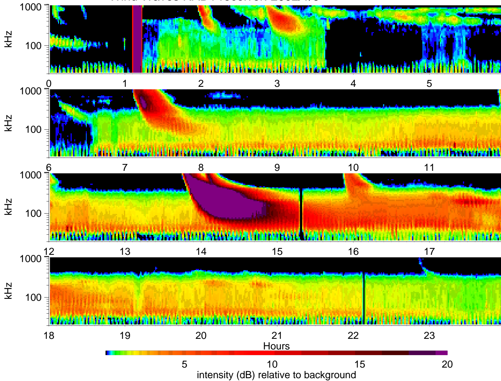
Wind Waves RAD1 receiver: 2002/1/6
