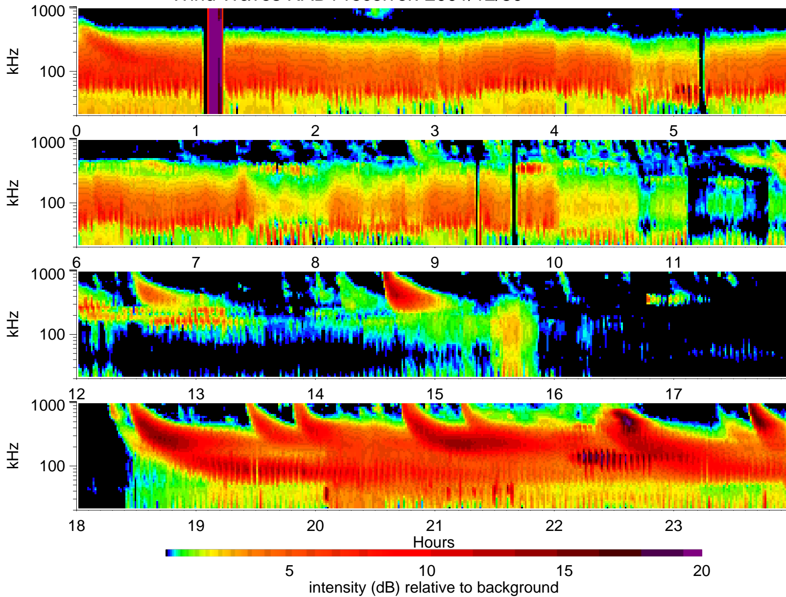
Wind Waves RAD1 receiver: 2001/12/30
