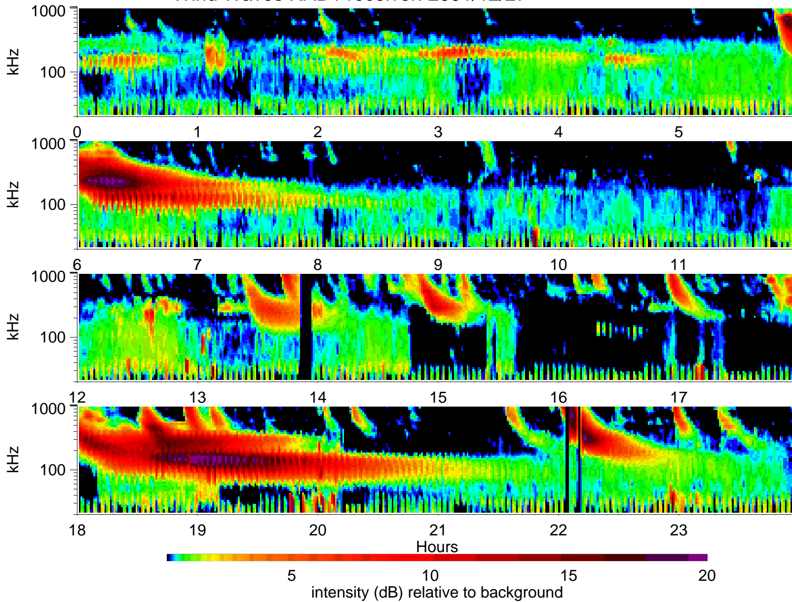
Wind Waves RAD1 receiver: 2001/12/27
