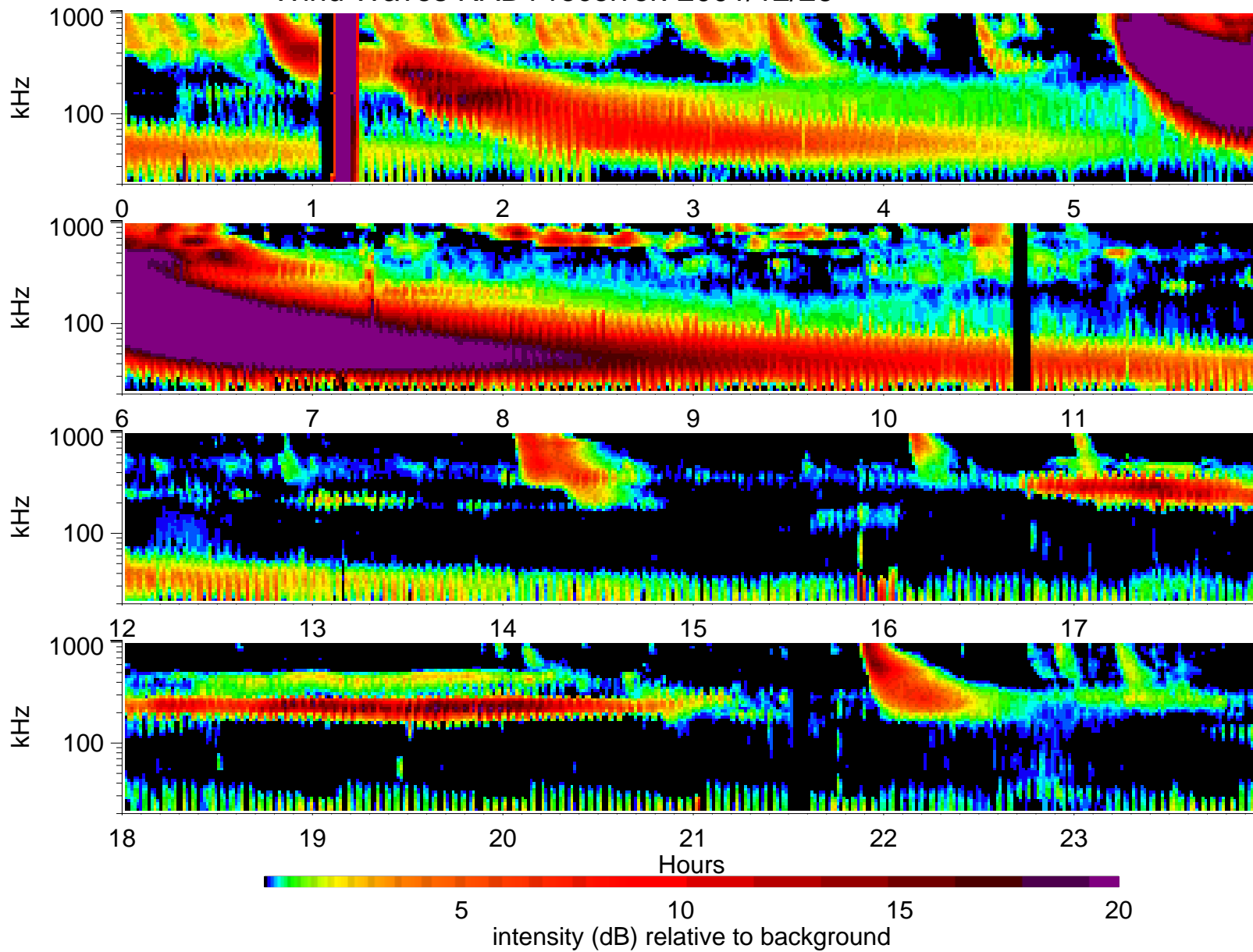
Wind Waves RAD1 receiver: 2001/12/26
