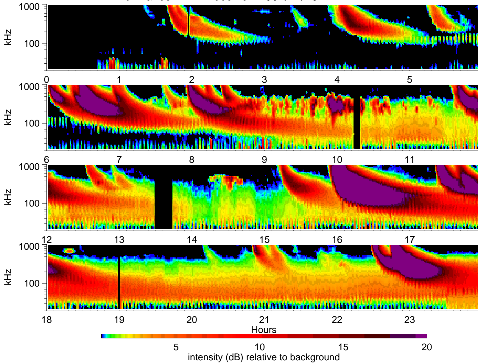
Wind Waves RAD1 receiver: 2001/12/23
