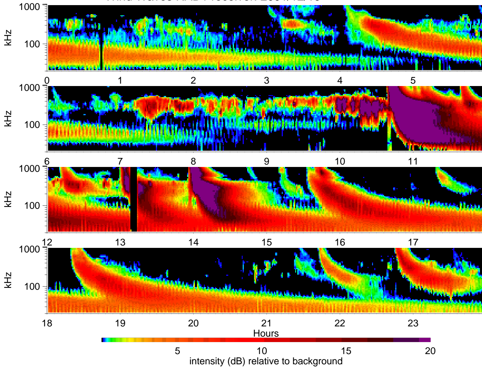
Wind Waves RAD1 receiver: 2001/12/19
